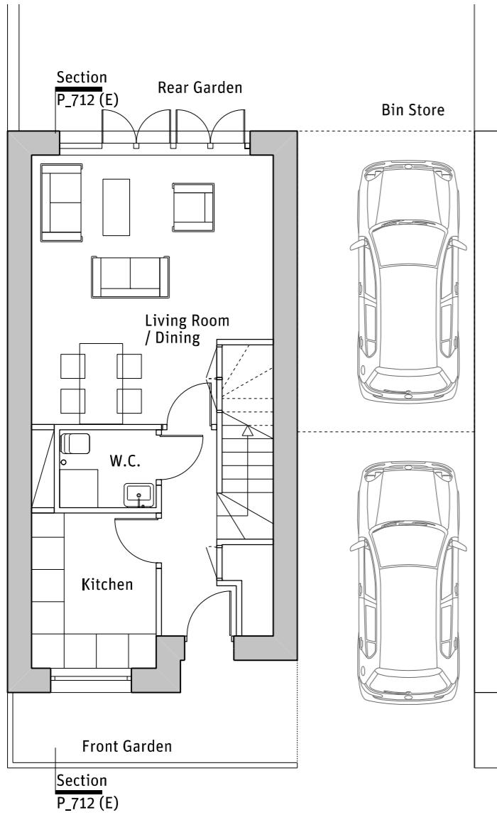
A GROUND FLOOR P_712 Plan 1:100
